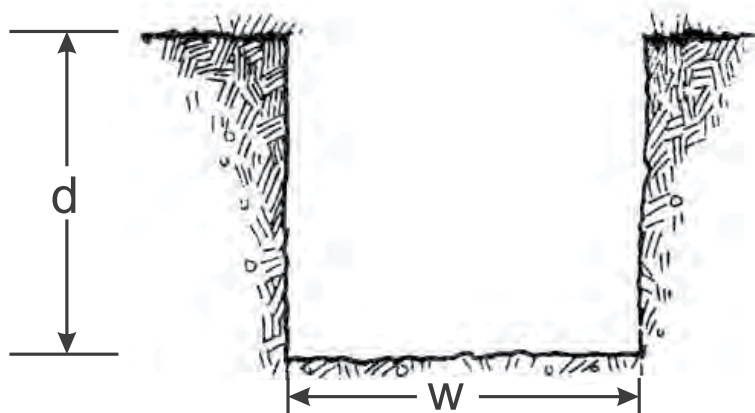
Open ( w > d ) Excavation
